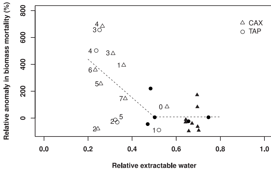
Figure 3. The anomaly in tree (more than 10 centimeters dbh) biomass with respect to background mortality rates at Caxiuanã National Forest (CAX) and Tapajós National Forest (TAP). The triangles represent CAX, the circles represent TAP, the filled symbols represent the control forest, and the open symbols represent throughfall exclusion (TFE)-treated forest. The number adjacent to each open symbol is the year of TFE treatment. The best-fit break point for the piecewise regression fit was at REW = .51 . For REW < .51 , y = 0.77 + 1404 (0.51 - x) ( p < .01 ); for REW > .51 the slope is not significantly different from zero.
