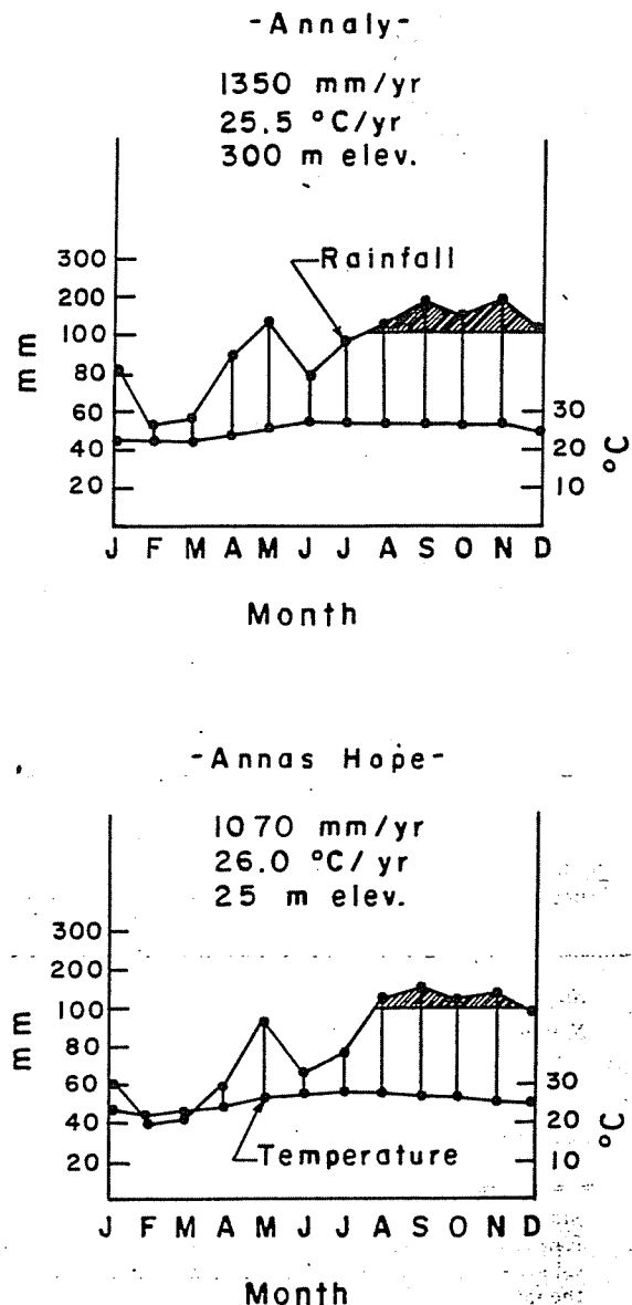
Fig. 2. Climatic diagrams for Annaly and Annas Hope, St. Croix.
