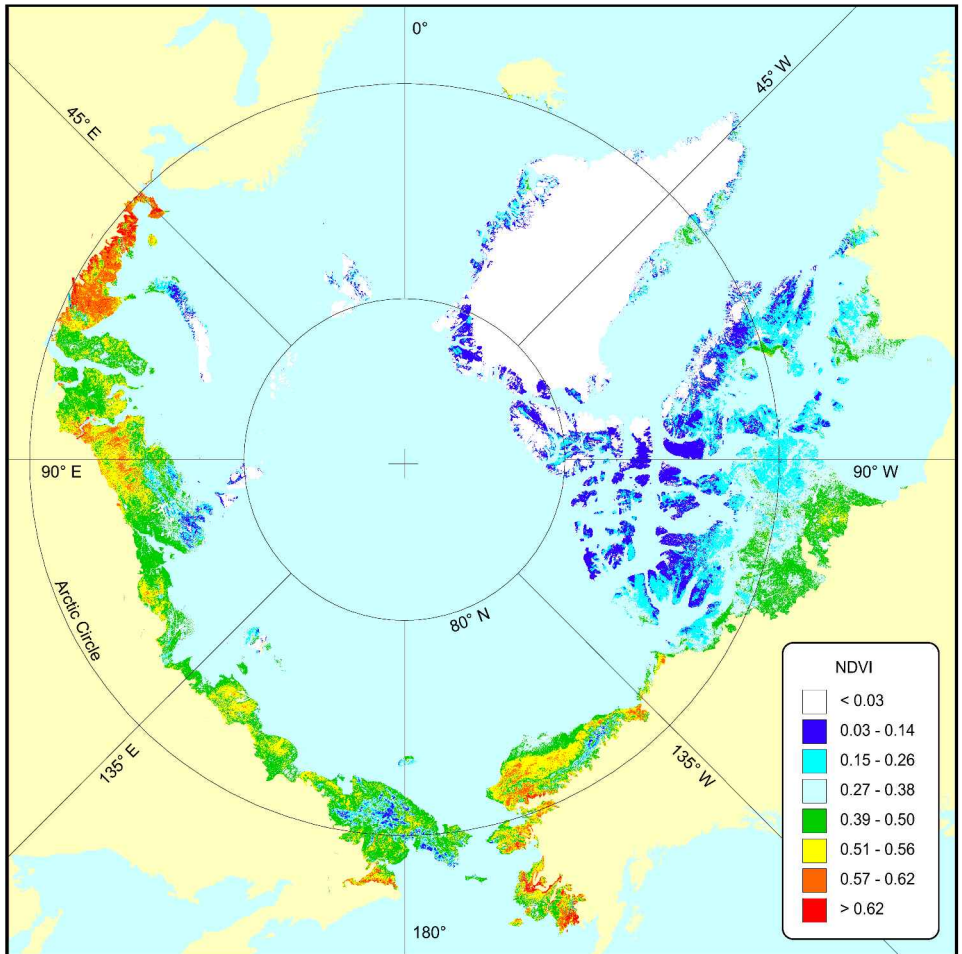
Figure 2. Maximum NDVI for the circumpolar Arctic derived from the same data as figure 5.
