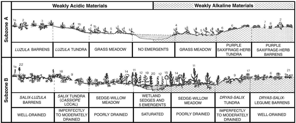
Figure 6. Vegetation on acidic and alkaline substrates in subzones A and B. Modified from Edlund and Alt (1989). Species shown are: 1, Luzula confusa ; 1b, L. arctica ; 2, Papaver radiculatum ; 3, Potentilla hyparctica ; 4, Alopecurus alpinus ; 5, Phippsia algida ; 6, Saxifraga oppositifolia ; 7, Poa abbreviata ; 8, Draba sp.; 11, Carex aquatilis var. stans ; 12, Pleuropogon sabinei ; 14, Eriophorum triste ; 15, E. scheuchzeri ; 17, Dryas integrifolia ; 18, Cassiope tetragona ; 19, Arctophila fulva ; 20, Hippuris vulgaris ; 21, Oxytropis arctobia ; 22, Hierochloa alpina .
