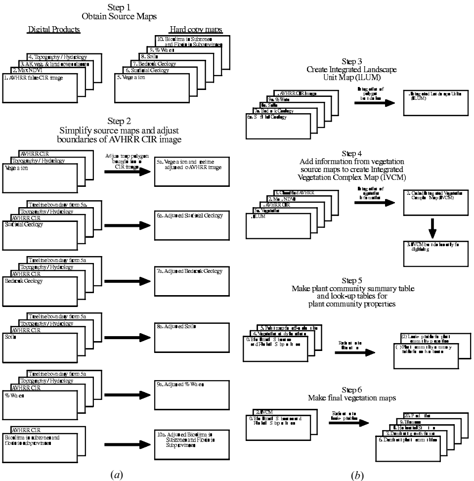
Figure 8. Six-step procedure for making the CAVM. See text for brief synopsis of each step. Summarized from Walker (1999).
