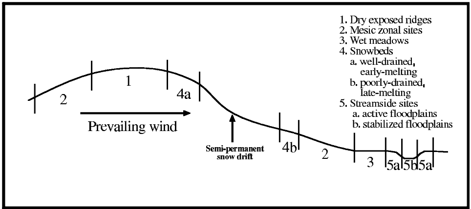
Figure 7. Conceptual mesotopographic gradient for arctic landscapes.
