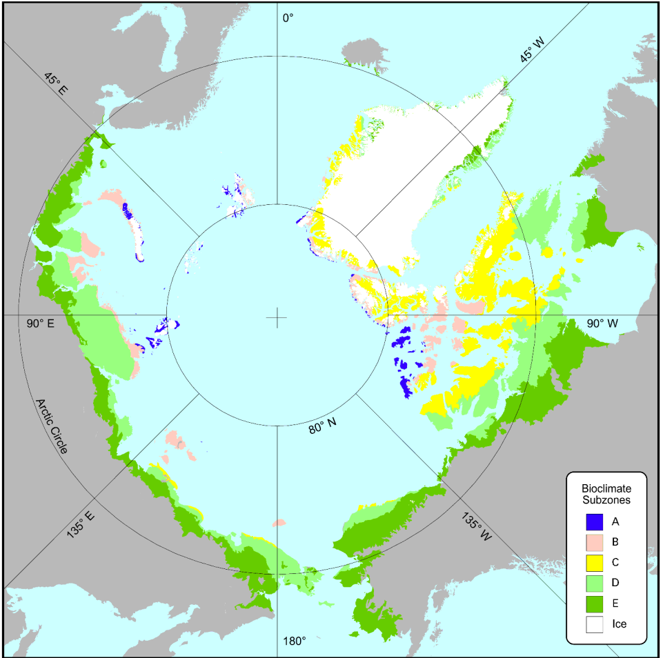
Figure 3. Bioclimatic subzones in the Arctic. Modified from Elvebakk et al. (1999).
