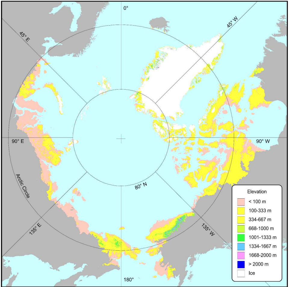
Figure 5. Topography of the circumpolar Arctic showing colour breaks corresponding to approximate altitudinal zonation boundaries. The environmental adiabatic lapse rate of 6°C per 1000m creates a shift in equivalent bioclimatic subzone about every 333-m elevation gain.
