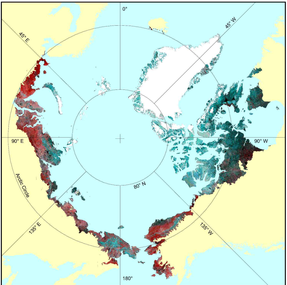
Figure 1. AVHRR-derived false colour-infrared image of the circumpolar Arctic. The image is derived from the pixels with highest NDVI among biweekly images from 1993 and 1995. The southern border of the CIR image is clipped to treeline, which was derived from the best available vegetation maps.
