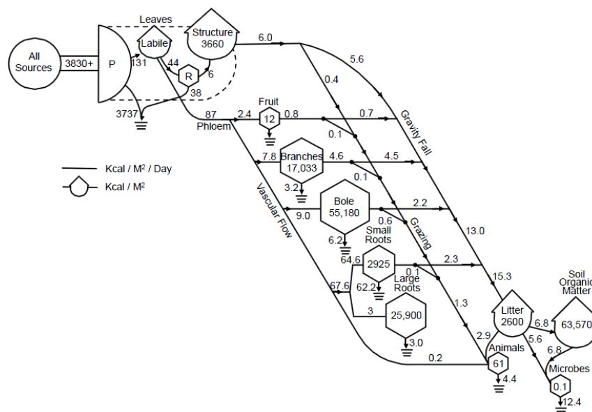
Figure 1. Carbon budget of a subtropical wet forest at El Verde, Puerto Rico [10] expressed in energy units (about 4 kcalories per g of vegetation material, because Odum used caloric equivalents of the various materials). The budget was constructed assuming steady state for the whole system. However, plants do exhibit greater production than respiration. Photosynthesis is P, R is respiration, structure refers to leaf biomass, and the symbols are those of the energy language of Odum [10]: bullet symbol represents photosynthesis, hexagons are consumer compartments, tanks are storages, the circle represents external energy inputs, the heat sinks are energy losses as a result of energy transformations, and lines represent the fluxes.
