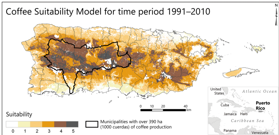
Fig. 1 Suitability index for coffee growth in Puerto Rico 1991–2010
