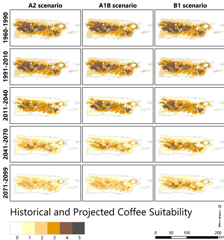
Fig. 2 Results of suitability model, 1960–2099 for IPCC SRES emission scenarios A2 (high), A1B (mid-low), and B1 (low) (Nakicenovic et al. 2000; Appendix 1) based on data from Henareh et al. (2016)
