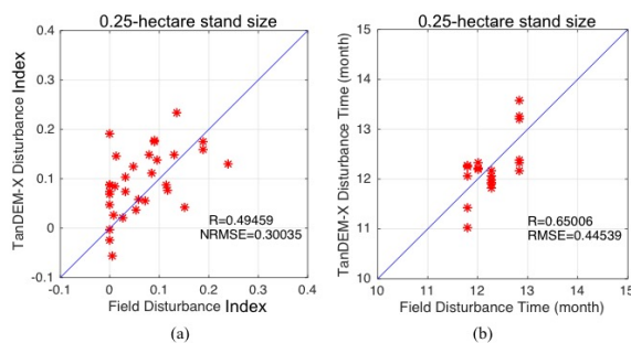
Fig. 4. (a) Scatterplot of TanDEM-X InSAR disturbance index and field disturbance index. (b) Scatterplot of TanDEM-X InSAR disturbance time and field disturbance time. Both the RMSE/NRMSE and the statistical R measure are shown with the stand size of 0.25 hectare.
