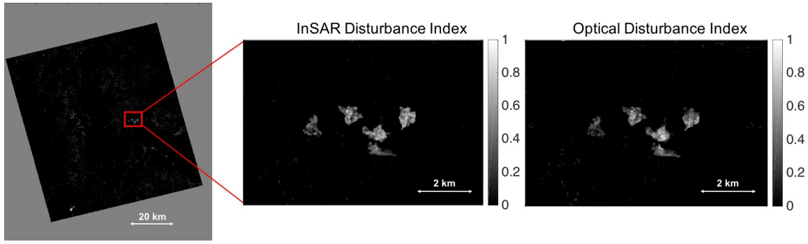
Fig. 1. (left) InSAR-derived disturbance index for the entire ALOS-1 InSAR image (84 km \times 72 km) over the ILCP site in Australia; (middle) blowup of the selective logging site for the InSAR disturbance index; (right) blowup for the optical disturbance index (derived from Landsat dense time series). 3 \times 3 median filter was applied in order to suppress the correlation sampling noise.
