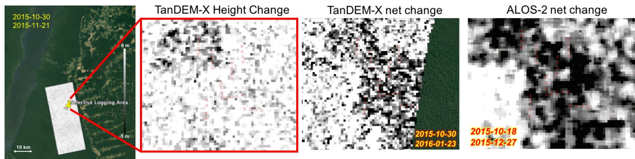
Fig. 3. (leftmost) phase-center height change between 20151030 and 20151121 for the entire TanDEM-X InSAR image ( 40 \text{ km} \times 16 \text{ km} ) over the Tapajos site in Brazil with the blowup of the selective logging site to the right; (second from the right) TanDEM-X phase-center height change between 20151030 and 20160123 (difference between before and after the disturbance event); (rightmost) ALOS-2 InSAR coherence component due to disturbance \gamma_{dist} (20151018–20151227). 3 \times 3 median filter was applied in all of the subfigures in order to suppress the correlation sampling noise. The greyscale is from -5 m (“black”) to 0 m (“white”) for all of the subfigures except the rightmost one, i.e., from 0 (“black”) to 1 (“white”).
