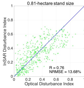
Fig. 2. Scatterplot of ALOS-1 InSAR disturbance index and Landsat optical disturbance index. Both the Normalized RMSE and the statistical R measure are shown with the stand size of 0.81 hectare.
