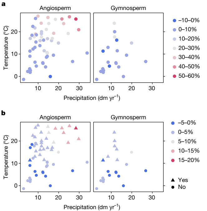
Fig. 2 | Decomposition rates and net insect effects in climate space. a, b , Annual mass loss of deadwood of native tree species, considering all possible groups of decomposers (uncaged treatment) ( a ) and annual mass loss attributed to insects (difference in mass loss between uncaged and closed-cage treatments), b , relative to the mean annual temperature and mean annual precipitation. Symbols indicate whether termites occur in the study areas. Points represent predicted values for angiosperm species at 55 sites and gymnosperm species at 21 sites based on a Gaussian generalized linear mixed log-link model for 2,533 logs with site-specific random effects and temperature, precipitation, treatment, host division, as well as their interactions, as fixed effects. Note that the lower sample size for gymnosperm species represents their global distribution.
